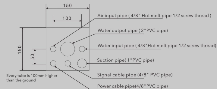
Pre-buried pipe distribution map
