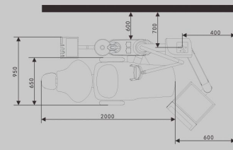
Exteranl floor-box installation sketch map
